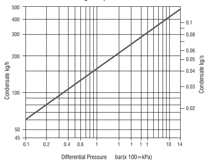
Discharge Capacities
